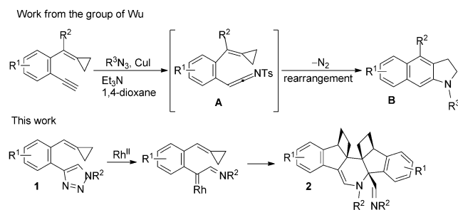
Scheme 1. Formation of N -heterocyclic compounds from 2-ethynylaryl MCPs and N -sulfonyl-triazole MCPs. Ts = 4-toluenesulfonyl.
